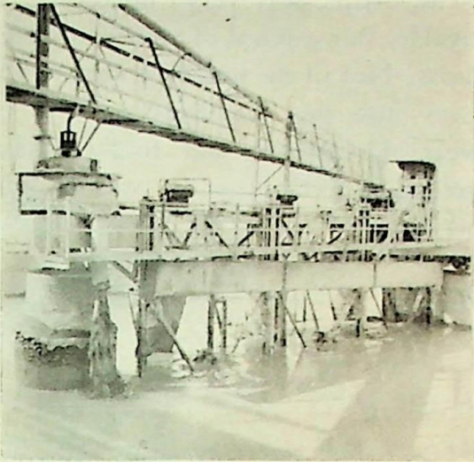
The mixture of lime-stone, clay and water in a Silo
